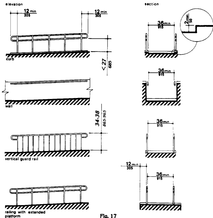
Fig. 17 Examples of Edge Protection and Handrail Extensions
