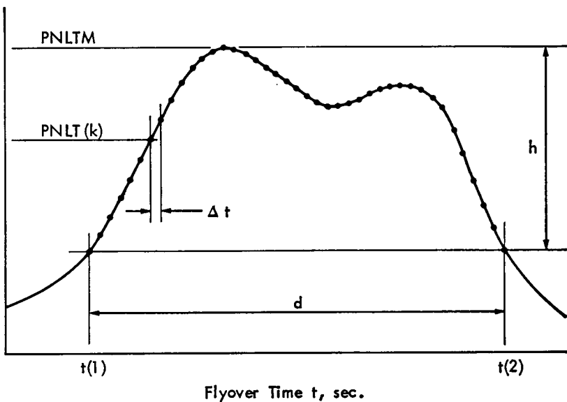
Figure B2. Example of Perceived Noise Level Corrected for Tones as a Function of Aircraft Flyover Time
